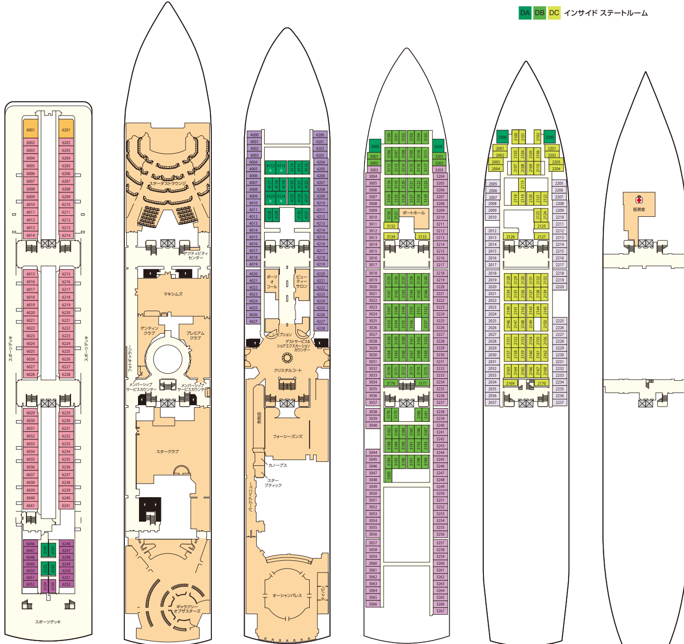
Deck 6 Deck 5 Deck 4 Deck 3 Deck 2 Deck 1
